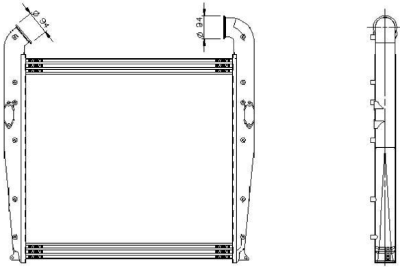
309018 825 x 797 x 62
