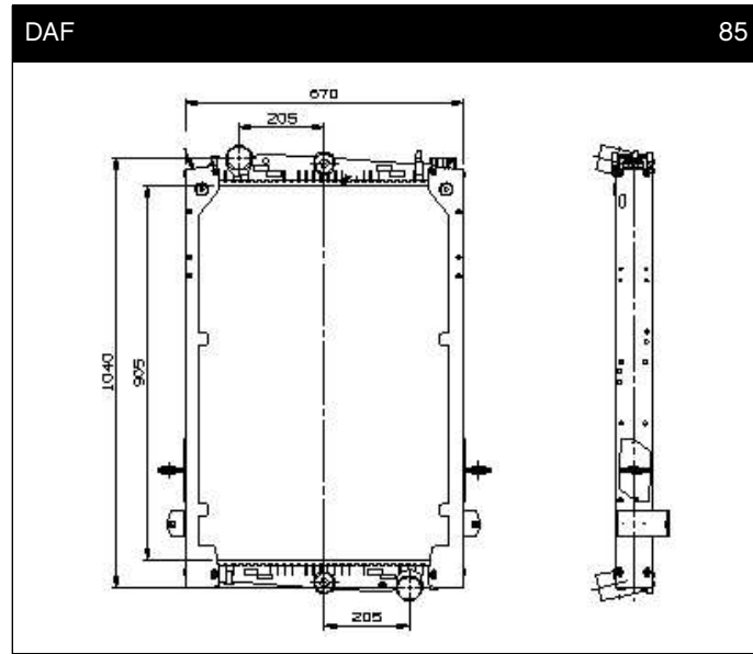
509586 905 x 648 x 56
