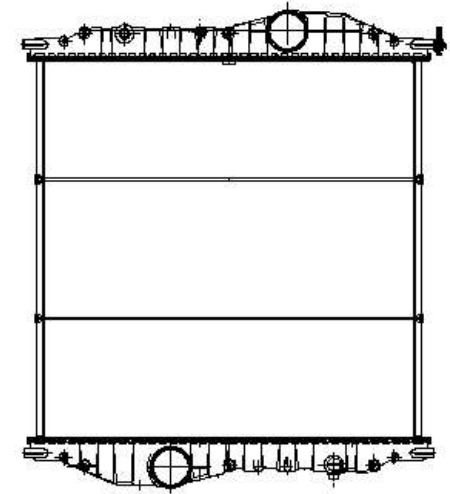
503465 650 x 665 x 53
