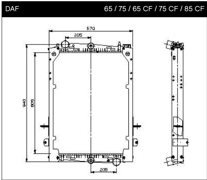
509585 805 x 648 x 56
