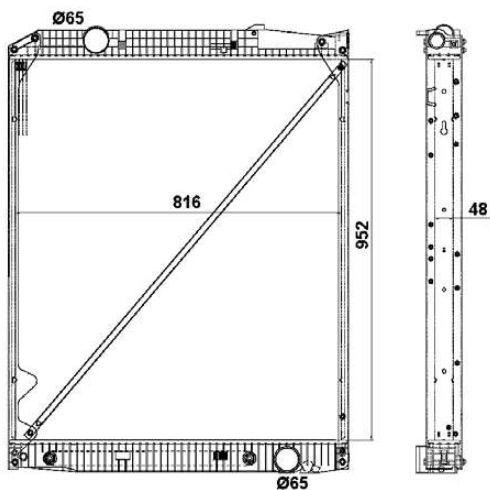
519577 952 x 829 x 48
