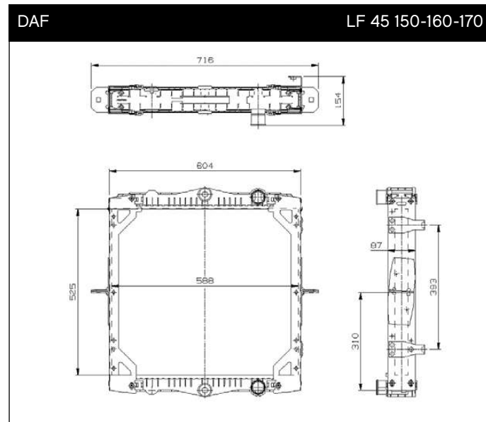
519569 525 x 588 x 56
