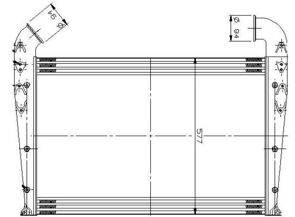
309191 837 x 577 x 62
